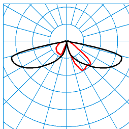
CS 19 100-AB2L/2200-730 2G1S (Tube4000mm) ■ C0 - C180 TX197073 ■ C90 - C270 DIN 5040: A20 UTE: 1,00 l CEN Flux Code: 26 63 96 100 100
