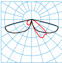
CS 19 100-AB2L/5100-730 4G1S (Tube4000mm) ■ C0 - C180 TX197089 ■ C90 - C270 DIN 5040: A20 UTE: 1,00 l CEN Flux Code: 27 65 96 100 100 0 0 0 0
