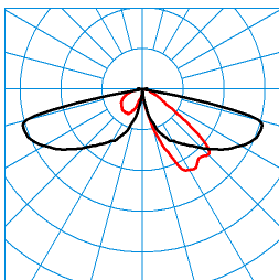
CS 19 100-AB2L-SLR1/5100-730 4G1S (Tube4000mm) ■ C0 - C180 TX197529 ■ C90 - C270 DIN 5040: A20 UTE: 1,00 l CEN Flux Code: 27 65 96 100 100 0 0 0 0
