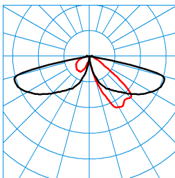
CS 19 100-AB2L/5100-740 4G1S (Tube4000mm) ■ C0 - C180 TX197097 ■ C90 - C270 DIN 5040: A20 UTE: 1,00 l CEN Flux Code: 27 65 96 100 100 0 0 0 0
