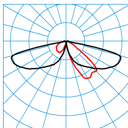
CS 19 100-AB2L-SLR1/5100-740 4G1S (Tube4000mm) ■ C0 - C180 TX197463 ■ C90 - C270 DIN 5040: A20 UTE: 1,00 l CEN Flux Code: 27 65 96 100 100 0 0 0 0
