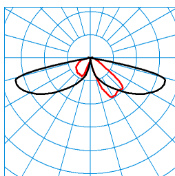
CS 19 100-AB2L/2200-740 2G1S (Tube4000mm) ■ C0 - C180 TX197081 ■ C90 - C270 DIN 5040: A20 UTE: 1,00 l CEN Flux Code: 26 63 96 100 100
