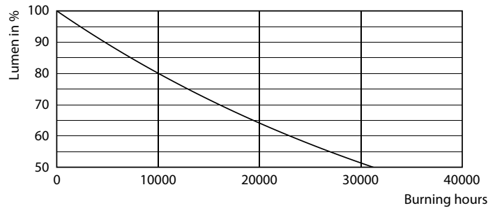
LEDBulb CLA SSW 60W E27 A60 Clear 827-822 ND
