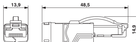
RJ45-Steckverbinder, IP20
